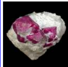
(4) Corundum Jagdalak Ruby Mine, Sorobi District, Konar, Afganistan
